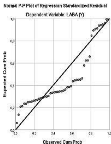
Gambar 1 Normal P-Plot
